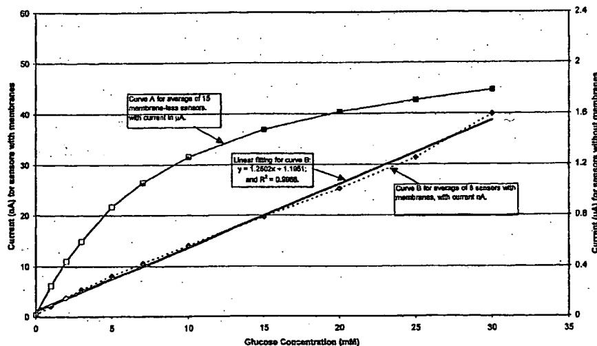
Calibration Curves at 37 °C
